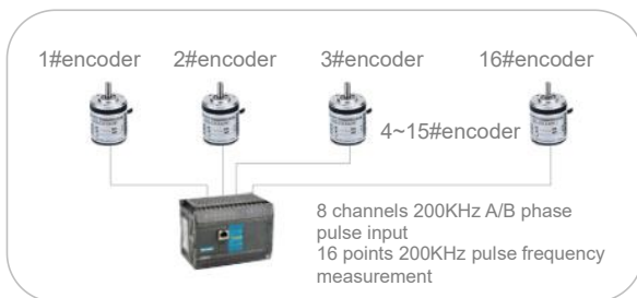
Haiwell PLC with 16 encoders
